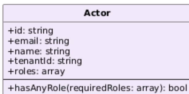
Figura 81: Classe: Actor
